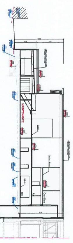
PC3.2 COUPE DINSSERTION - MAINTENANCE ech:1/200
